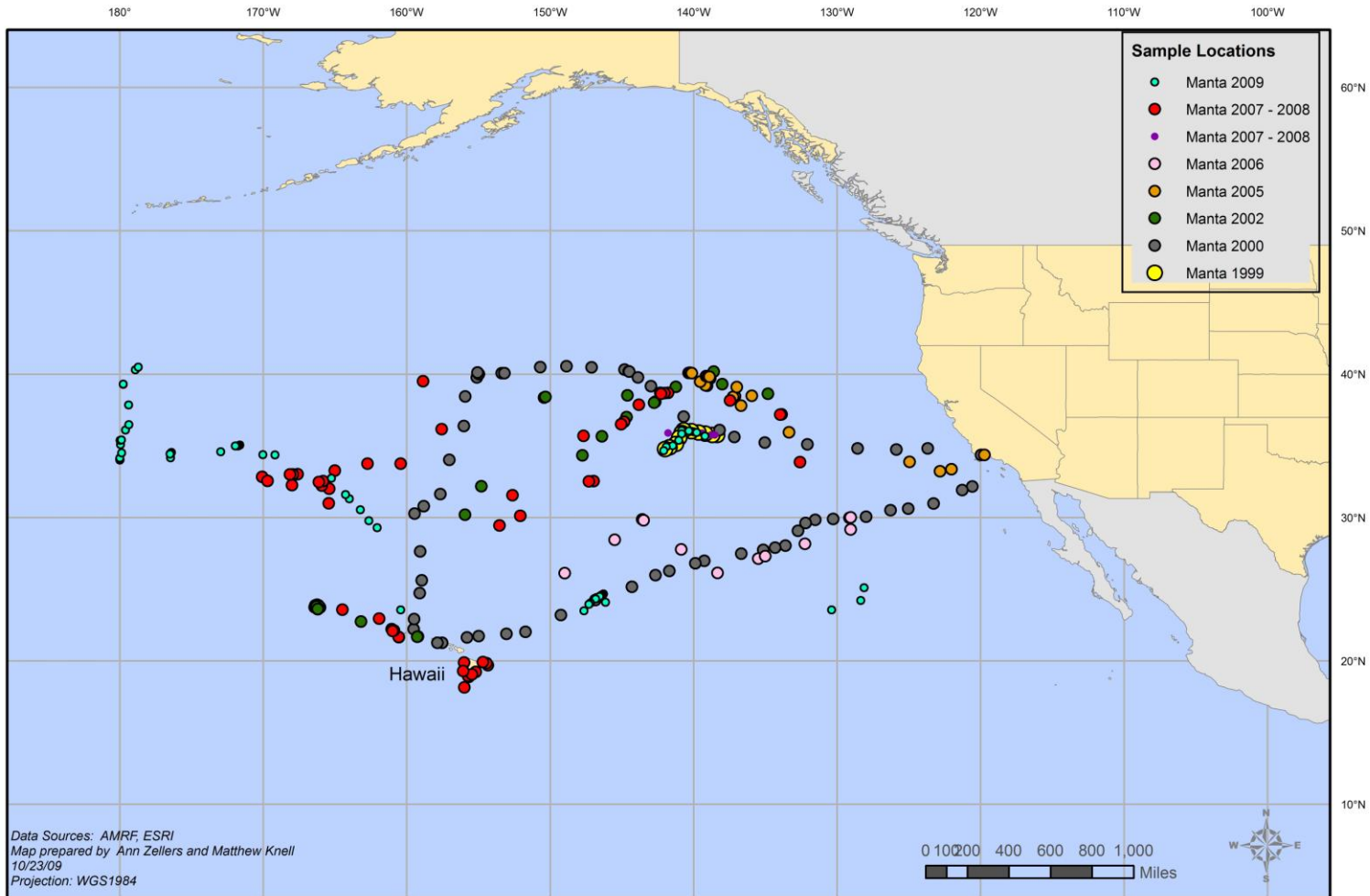
Plastic Marine Debris Surface Sample Locations North Pacific Gyre 1999 - 2009
